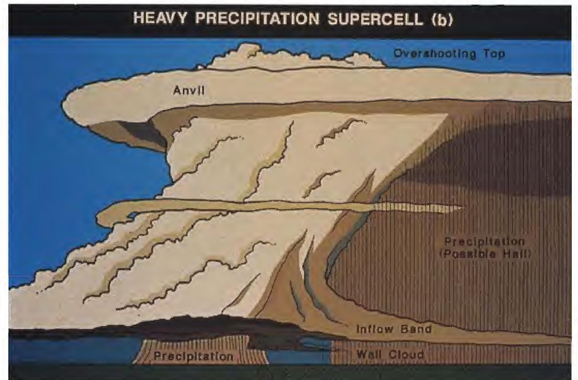
Figure 38: Schematic diagram of a high-precipitation supercell.
